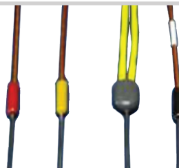
MOLDED TRANSITION THERMOCOUPLE
