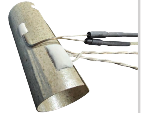
NON-SHEATHED HI-TEMP FORMED MICA
